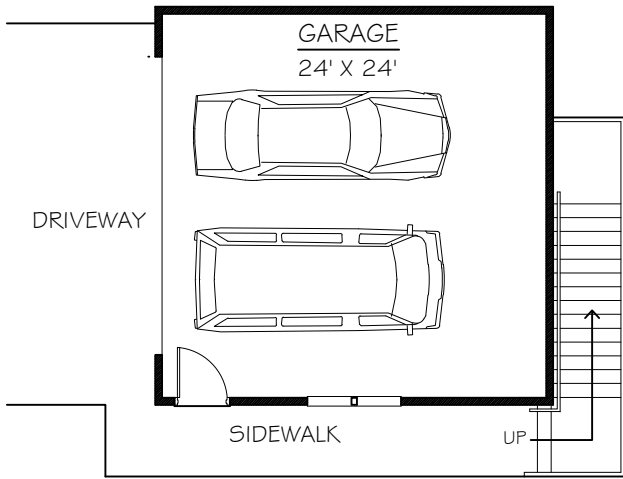
GARAGE FLOOR PLAN 576 SF
