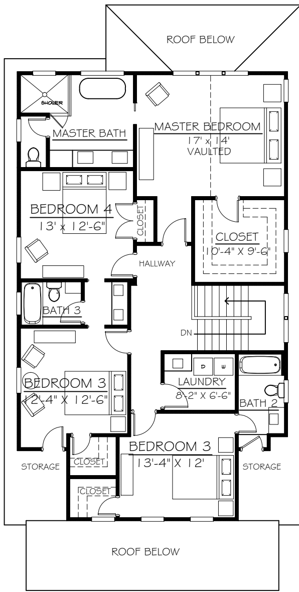
SECOND FLOOR
